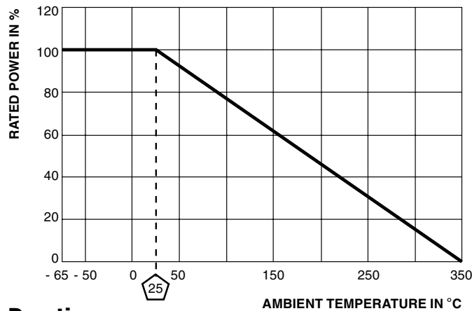
Derating
